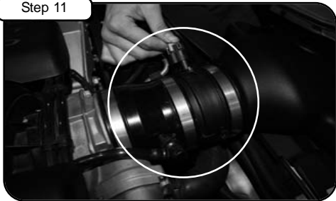
Re-connect MAF sensor harness and vacuum line.
