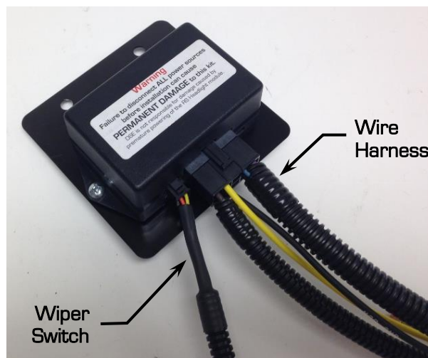
Figure 29 – Connect Wiper Switch & Harness to Module
