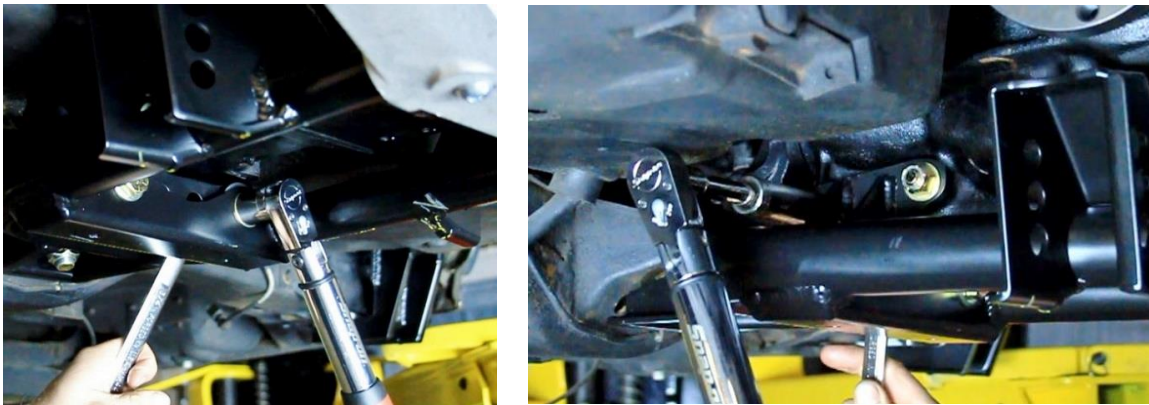
Figure 91 – Torque Lower Differential Bracket
