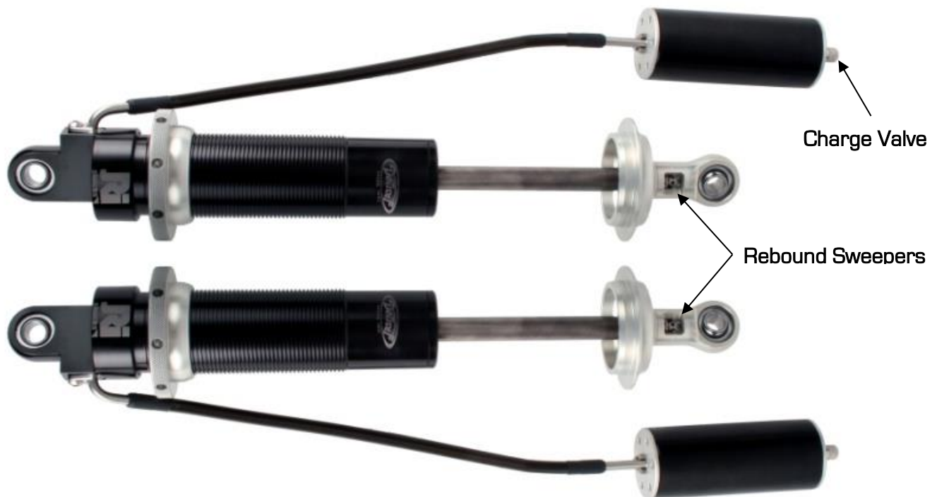
Figure 119a – Detroit Speed Double Adjustable Shock w/Remote Canister
