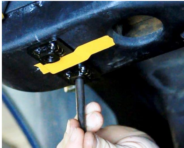
Figure 60 – Transfer Punch Nut Plate Location
