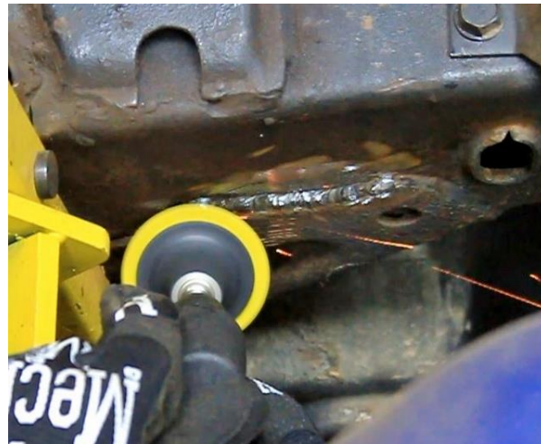
Figure 26 - Weld & Grind Gusset
