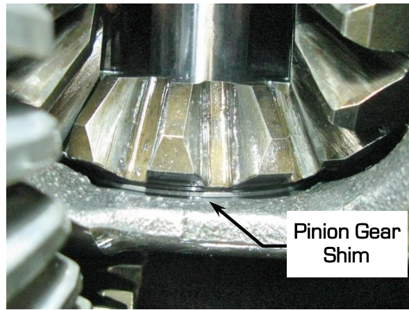
Figure 68 – Pinion Gear Shim
