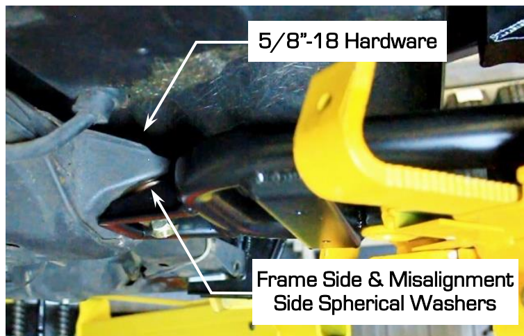
Figure 39 – Bolt Lower Cradle to Frame
