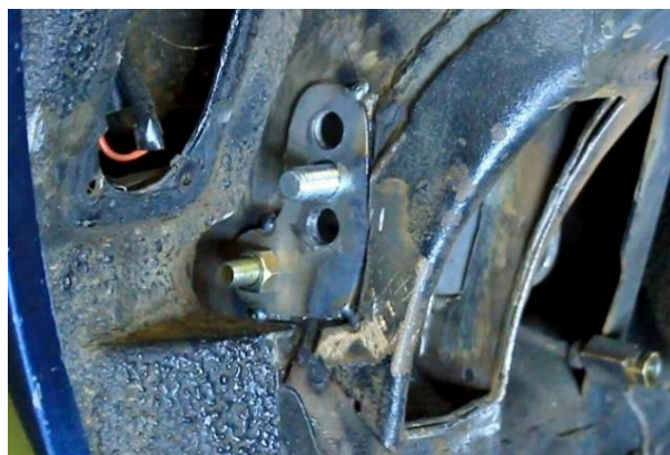
Figure 18 – Locate Inner Doubler Plate
