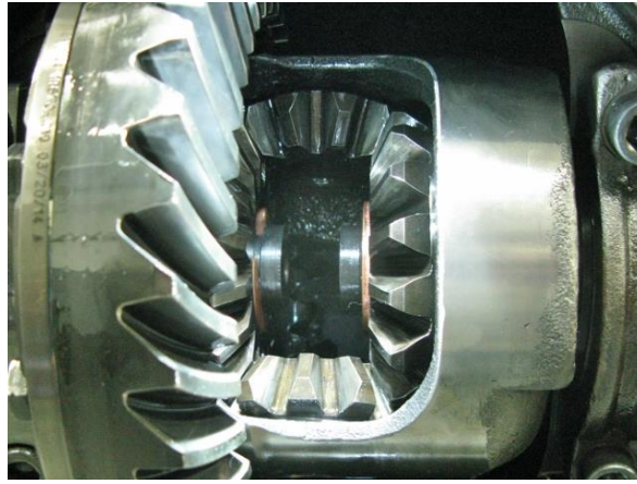
Figure 72 – Install Detroit Speed Stubs Axles
