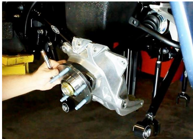
Figure 101 – Install Rear Upright to Outer CV Joint
