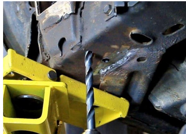
Figure 27 - Drill Trailing Arm Bracket Mounting Locations
