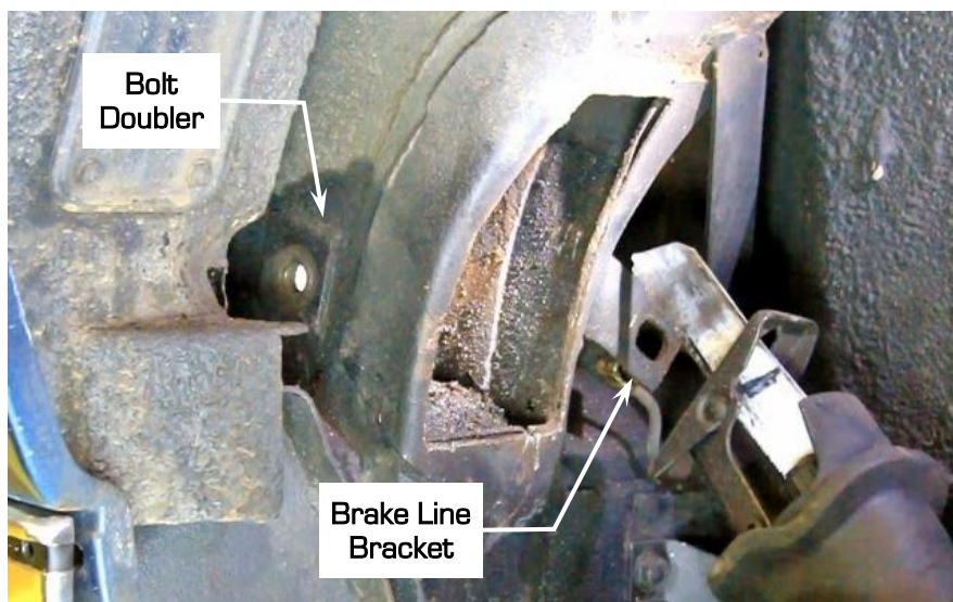
Figure 4 – Remove Park Brake Cable Bracket and Trailing Arm Bolt Doubler
