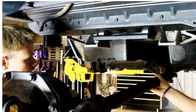
Figure 85 – Install Rear Differential Assembly
