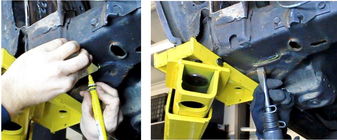
Figure 25 - Trim Frame Gusset
