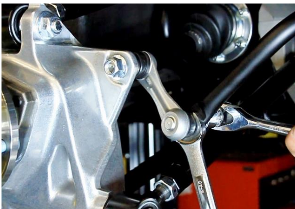
Figure 105 – Install Sway Bar End Link Assemblies
