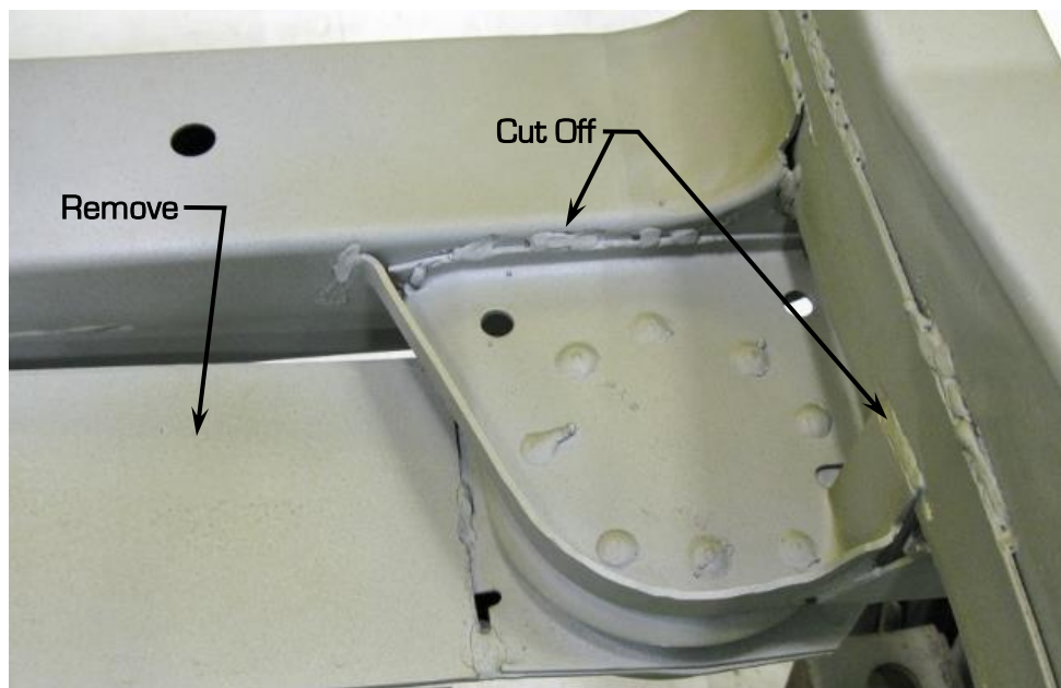
Figure 2 – Remove Frame Crossmember Brackets
