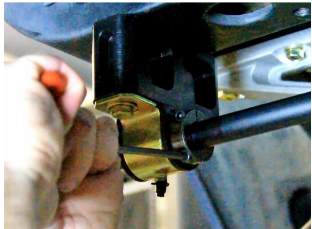
Figure 99 – Center Sway Bar and Install Split Lock Collars
