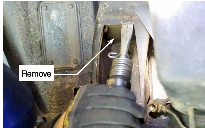
Figure 5 – Remove Doubler Plate
