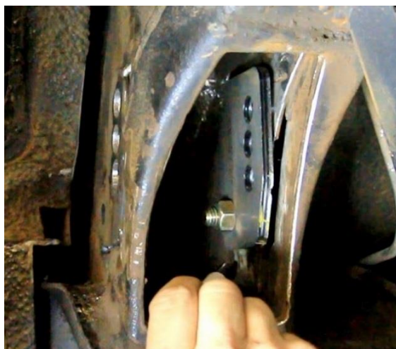
Figure 15 - Level Drill Guide
