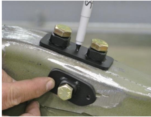
Figure 44 – Framerail Nut Plate Location
