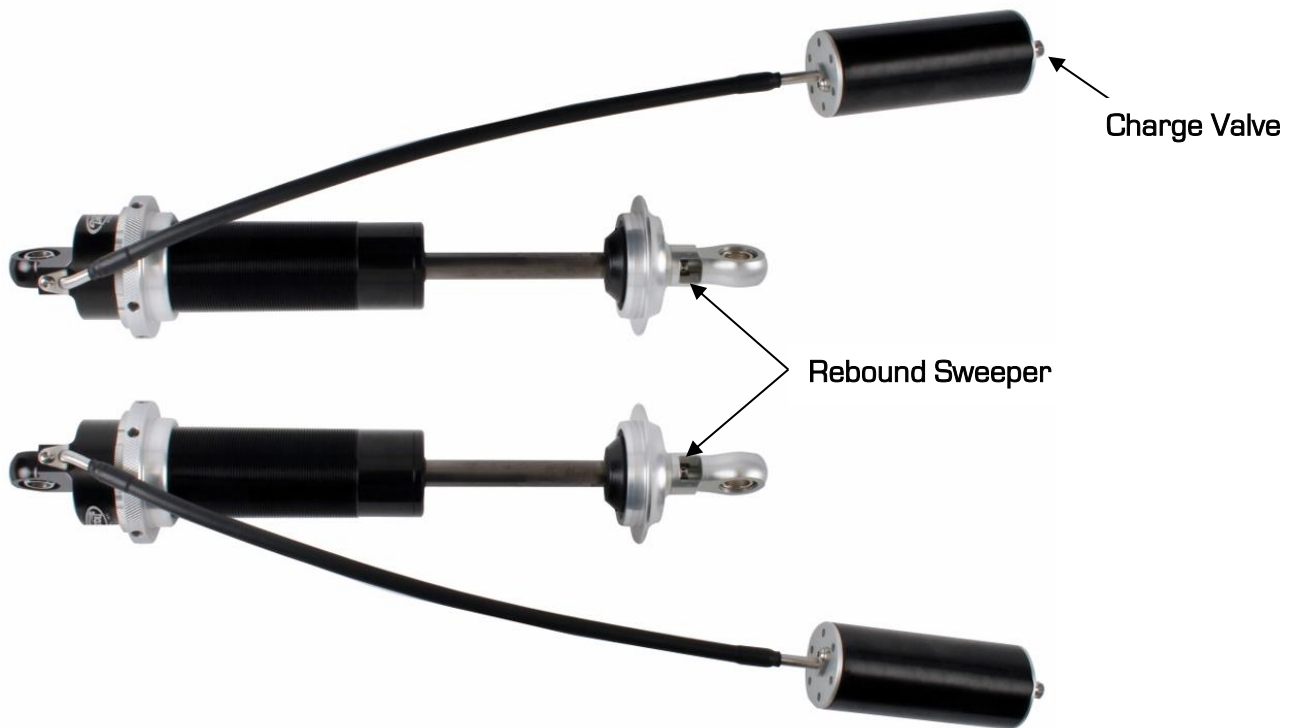
Figure 118a- Detroit Speed Single Adjustable Shock
