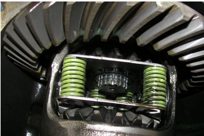
Figure 69 – Remove Snap Rings
