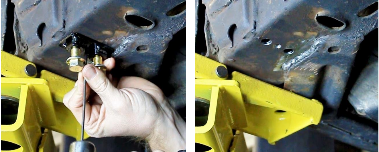
Figure 28 – Trailing Link Bracket Nut Plate
