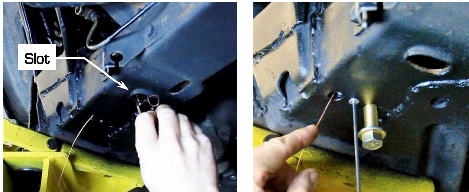
Figure 30 – Install Trailing Link Bracket Nut Plate
