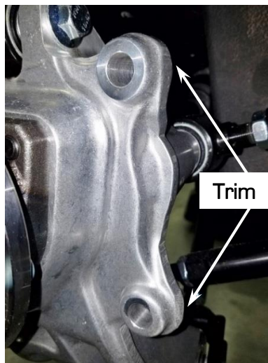
Figure 115 – Trim Upright
