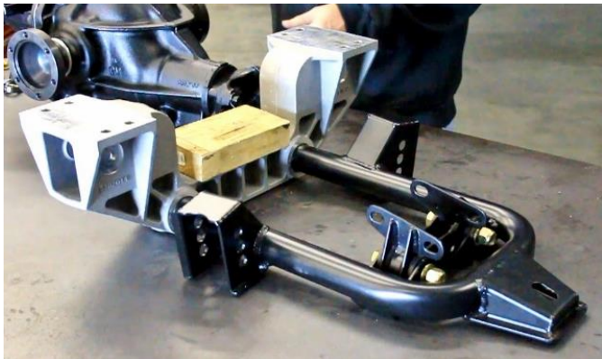
Figure 77 – IRS Lower Cradle/Rear Differential Assembly
