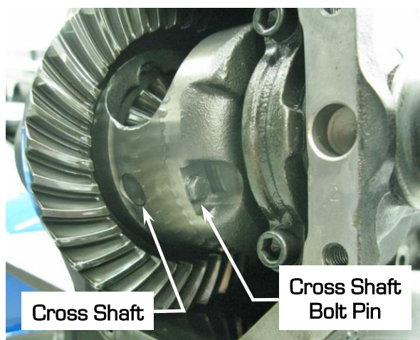
Figure 67 - Cross Shaft & Cross Shaft Bolt Pin
